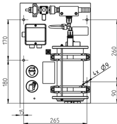
Abb. 7: Wandmontage Connex TCD PP
