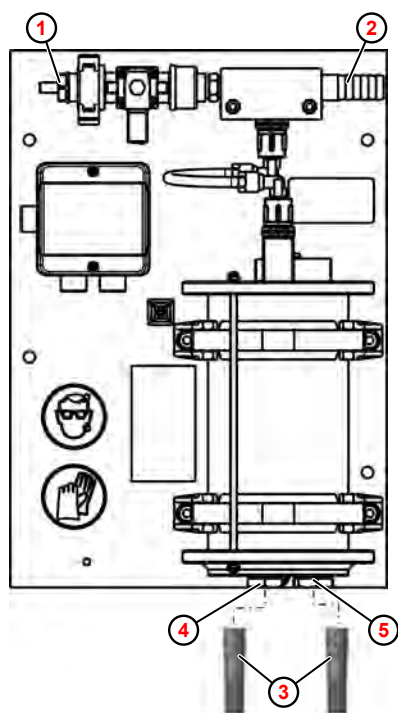
Fig. 9: Hydraulic installation
