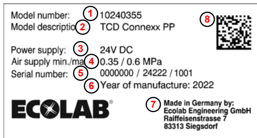
Fig. 17: Type plate
