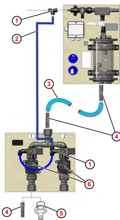
Fig. 10: Connecting the Connexx TCD valve distributor
