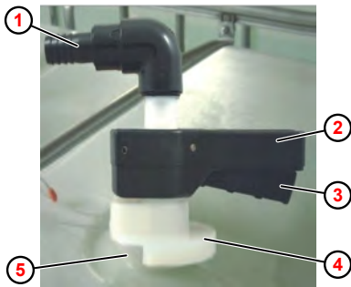
Fig. 3: ‘Click & Plug’ - connection coupling
