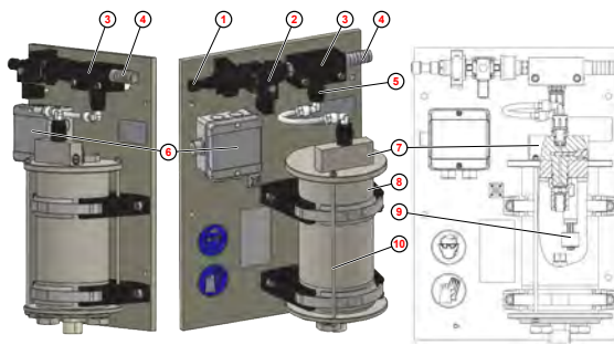
Fig. 5: Setup
