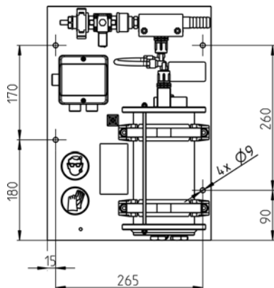
Fig. 7: Wall mounting Connex TCD PP
