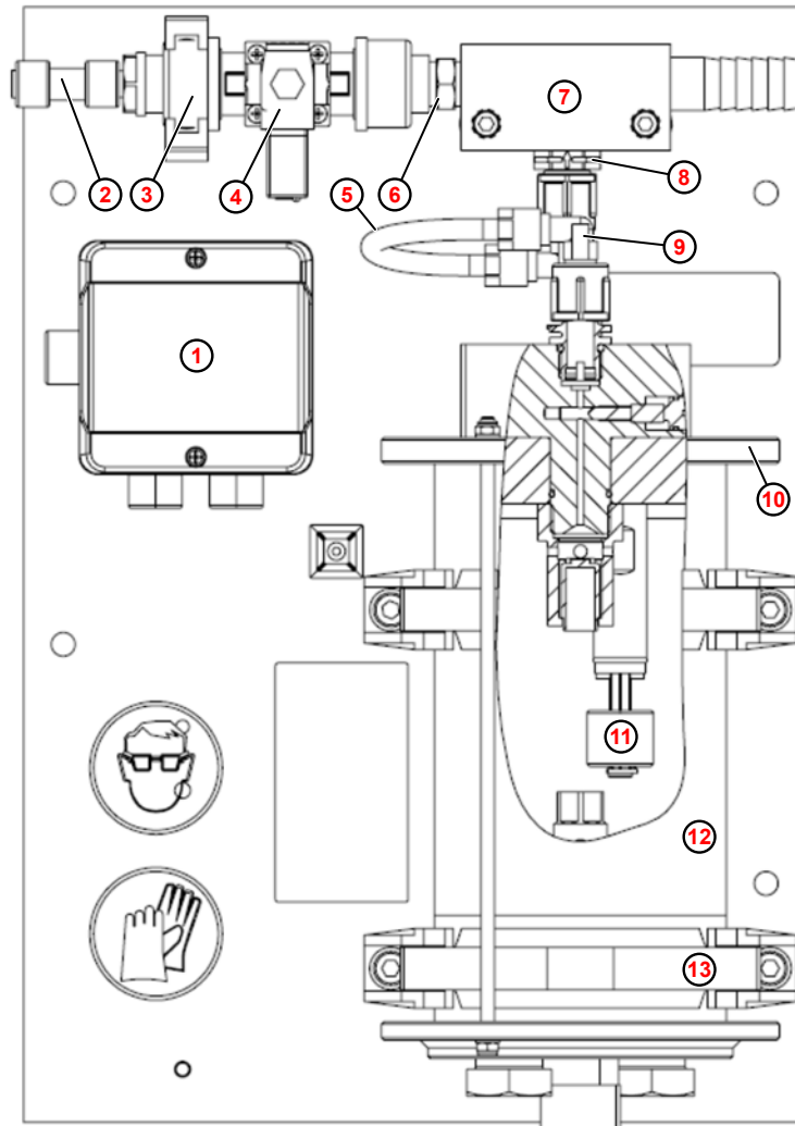
Fig. 16: Spare parts
